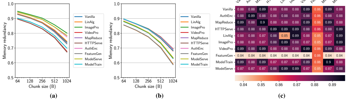
Figure 1. Memory redundancy in serverless workloads. Redundancy between sandboxes of the same function w.r.t. chunk size (a) with ASLR disabled and (b) with ASLR enabled. (c) Cross function redundancy - redundancy of functions on vertical axis w.r.t. those on horizontal axis with 64B chunk size.
